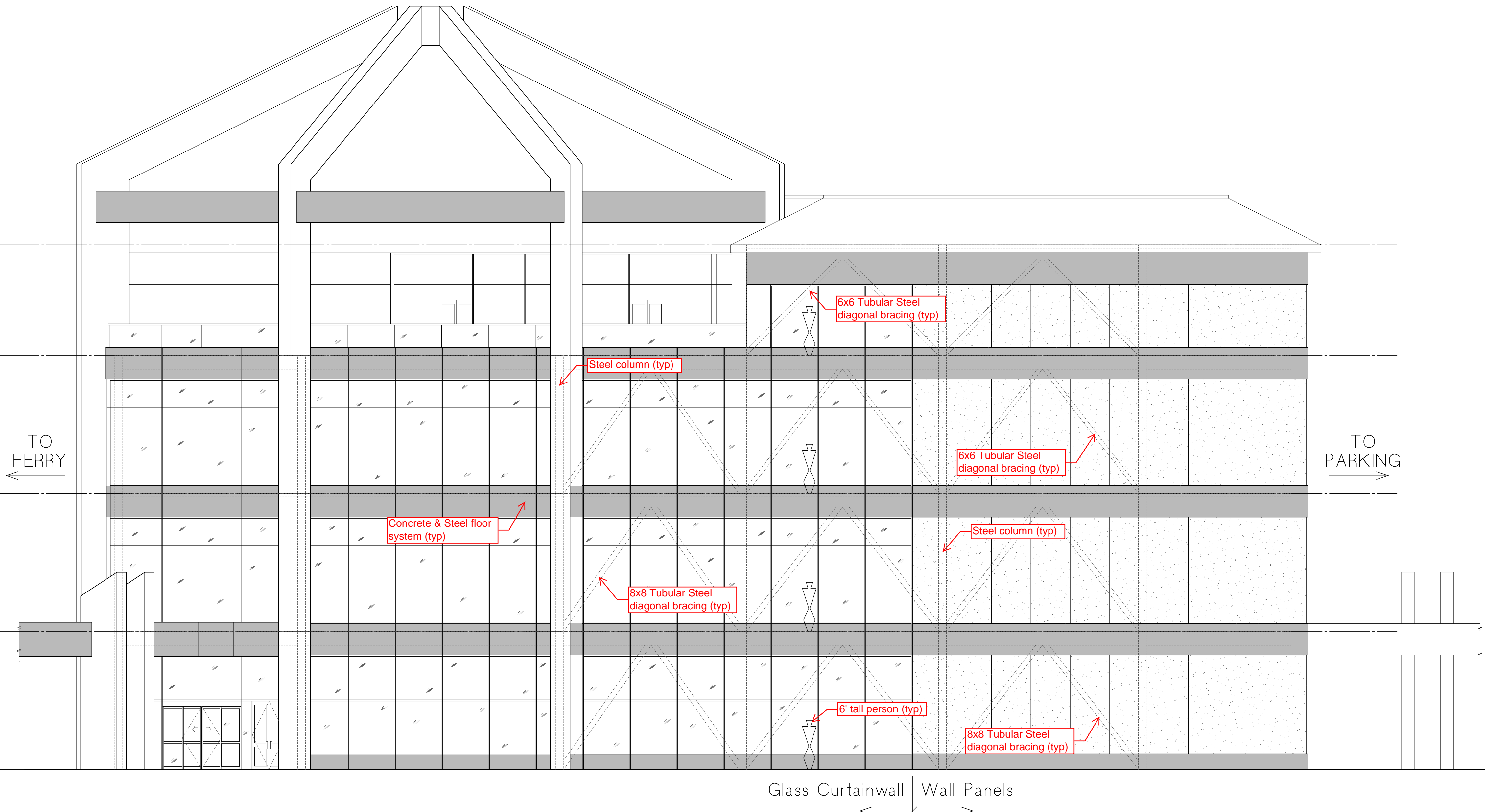
PROPOSED ELEVATION #3 SCALE: 1/8" = 1'-0"
